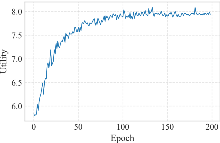
DSCI_Convergence Convergence
