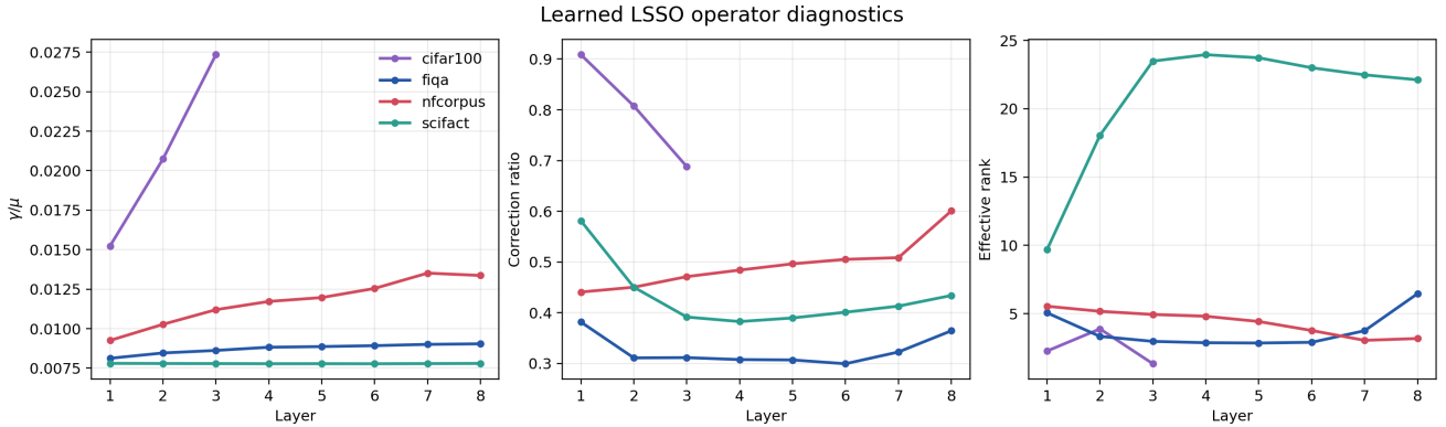
Figure 1: Layer-wise LSSO diagnostics from trained LSSO-r32 checkpoints.
