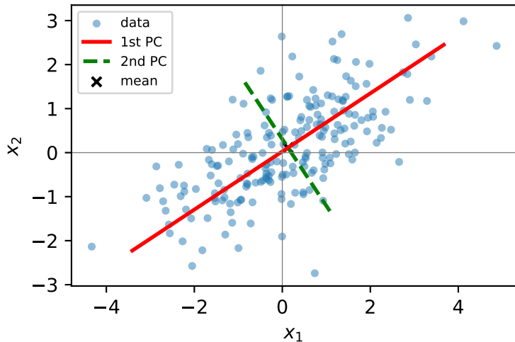
Anisotropic 2D data
