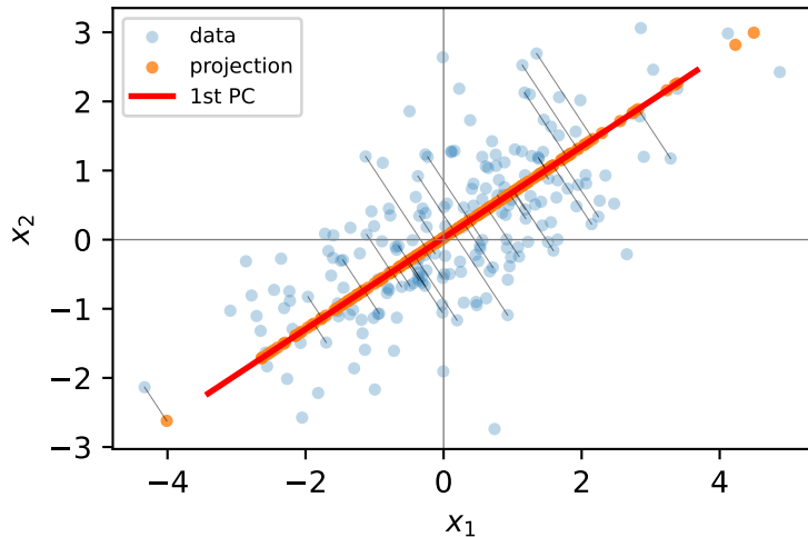
Projection onto 1st PC
