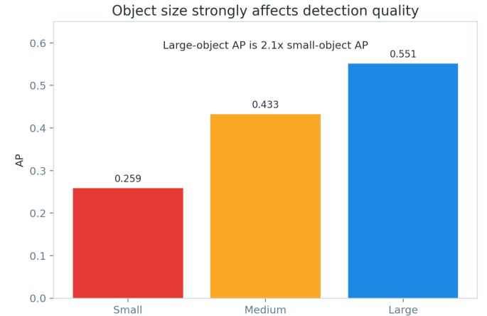
Fig. 3. AP gap across object sizes: small (APS), medium (APM), and large (APL) objects.
