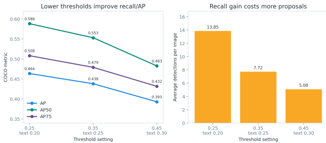
Fig. 7. Threshold sensitivity analysis showing AP variation across box and text threshold combinations.
