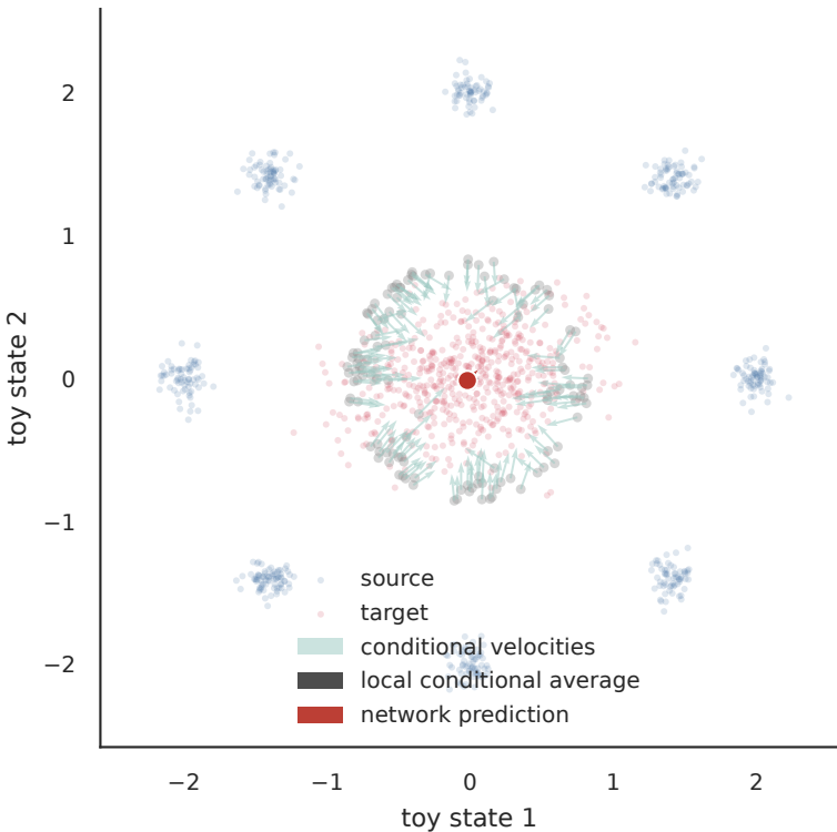
Conditional velocities collapse to a marginal vector
