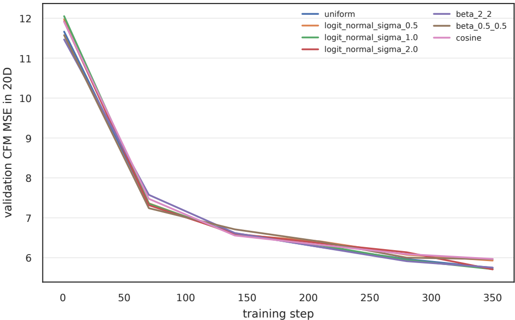
Time sampling ablation: validation velocity-regression MSE
