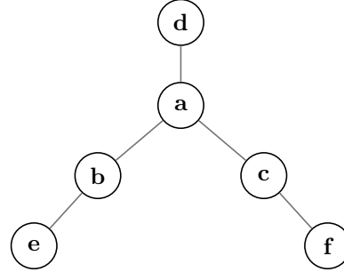
G' : a tree on 6 vertices
