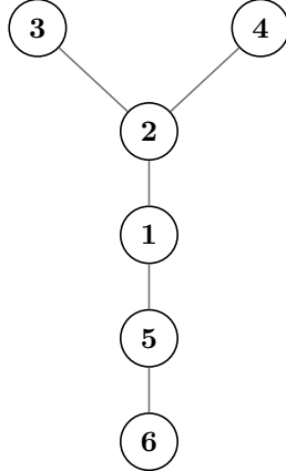
G : a tree on 6 vertices
