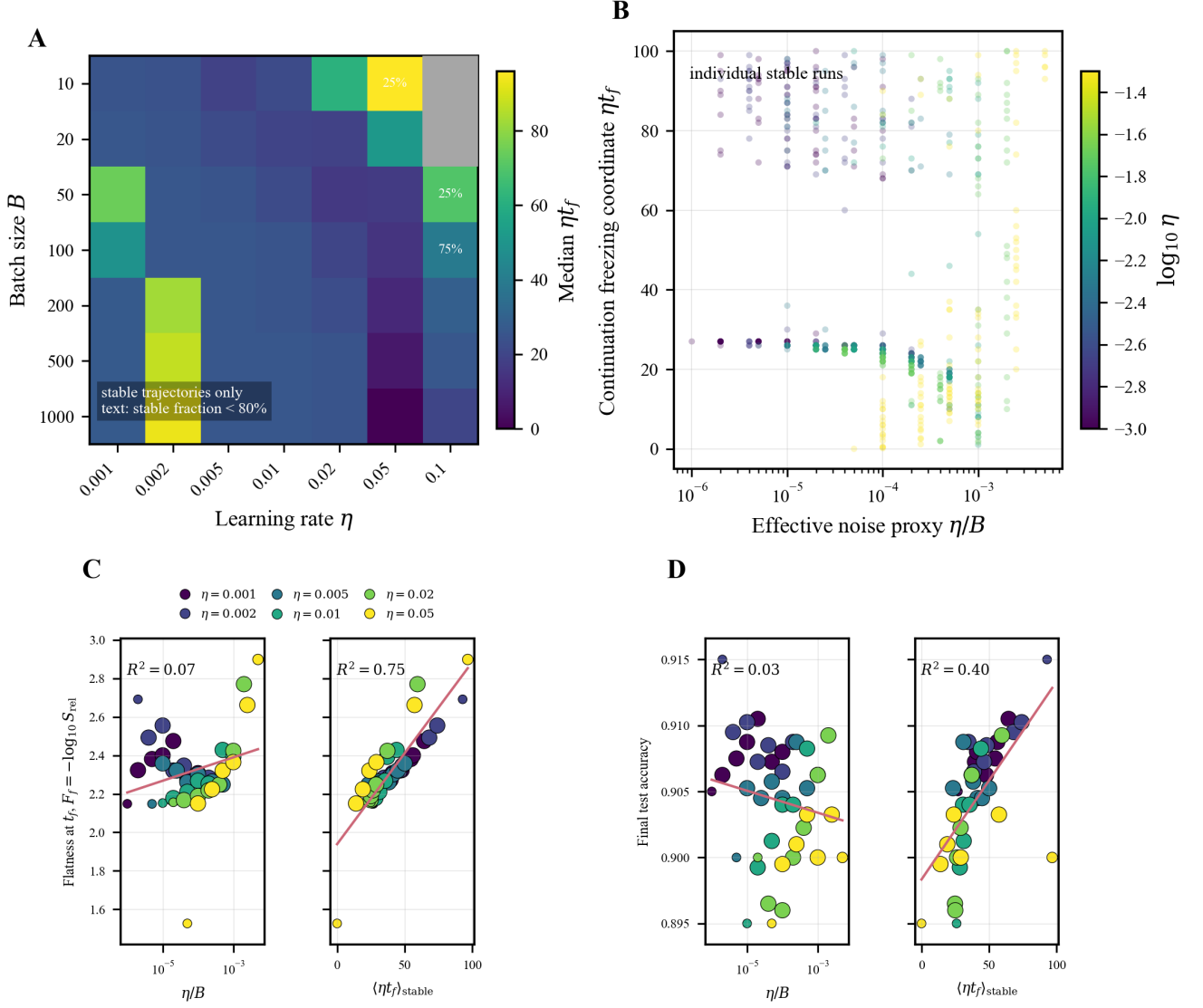
FIG. 2. Freezing time organizes basin commitment and the geometry observed at commitment. (A) Median continuation-based freezing coordinate \eta t_f across batch size and learning rate; gray cells indicate conditions without final-converged stable trajectories, and text marks stable fractions below 80%. (B) Individual final-converged stable runs show the distribution of \eta t_f across the effective noise proxy \eta/B . (C) Freezing-time flatness F_f = -\log_{10} S_{\text{rel}}(\theta_{t_f}) , measured at the checkpoint corresponding to t_f , compared with \eta/B (left) and with (\eta t_f)_{\text{stable}} (right). (D) Final test accuracy compared with the same two organizing variables. Point colors indicate learning rate; comparison panels omit the highest-learning-rate sweep and include continuation-stable trajectories that converge at the final checkpoint.
