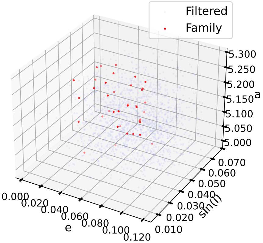
Osculating Orbital Elements
