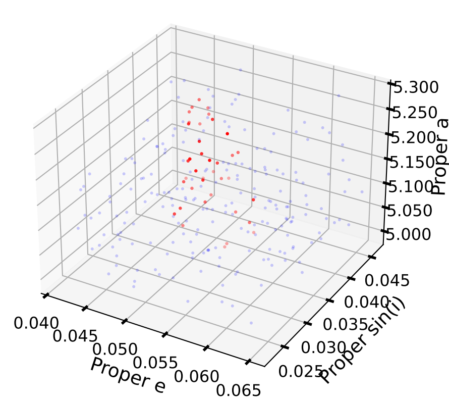
Proper Orbital Elements
