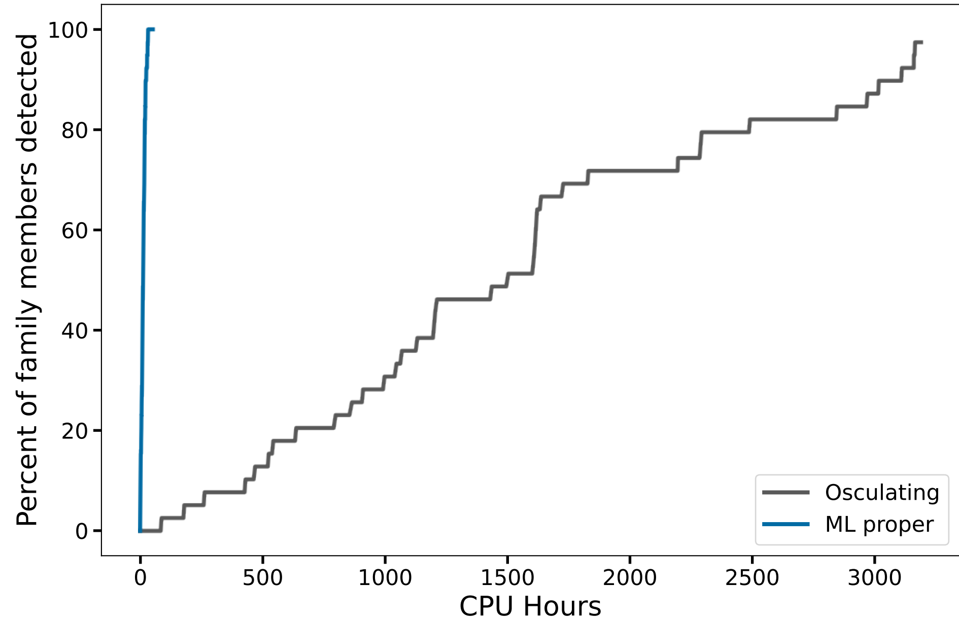
Detection Rate vs. CPU Hours
