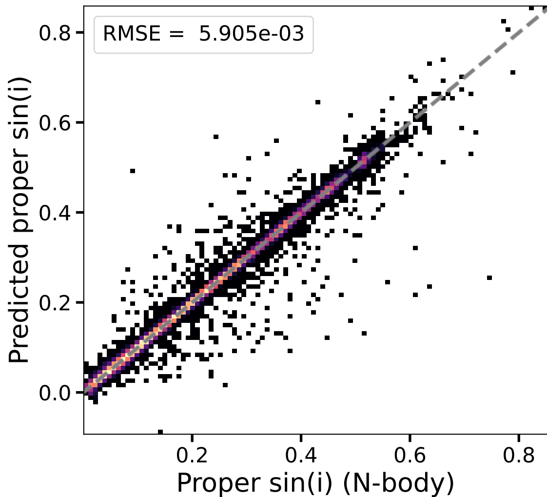
N-body vs Predicted proper sin(i)
