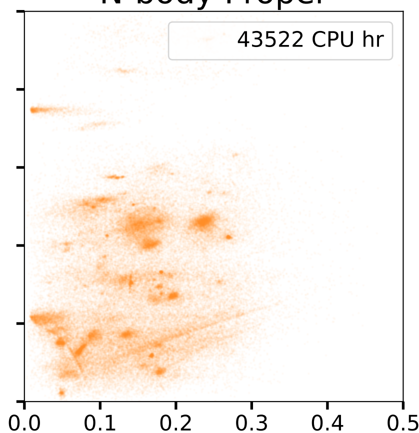
N-body Proper
