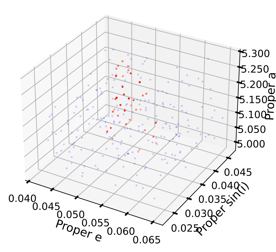
Proper Orbital Elements
