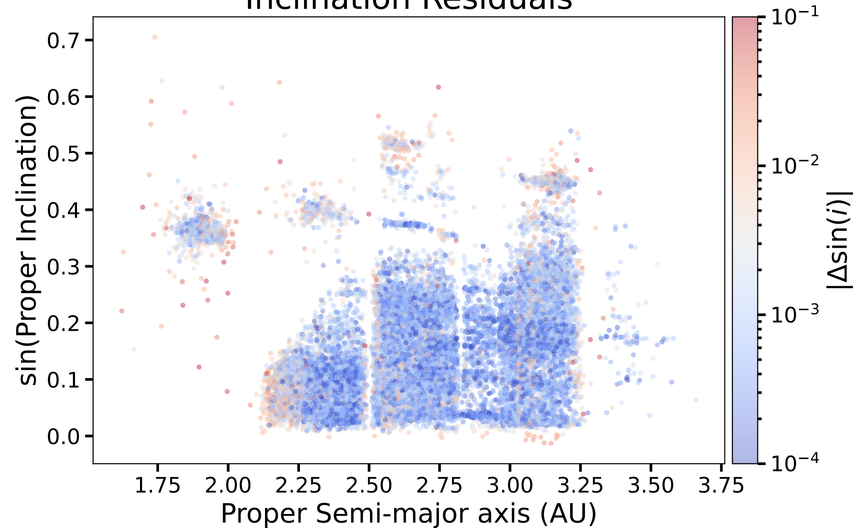
Inclination Residuals
