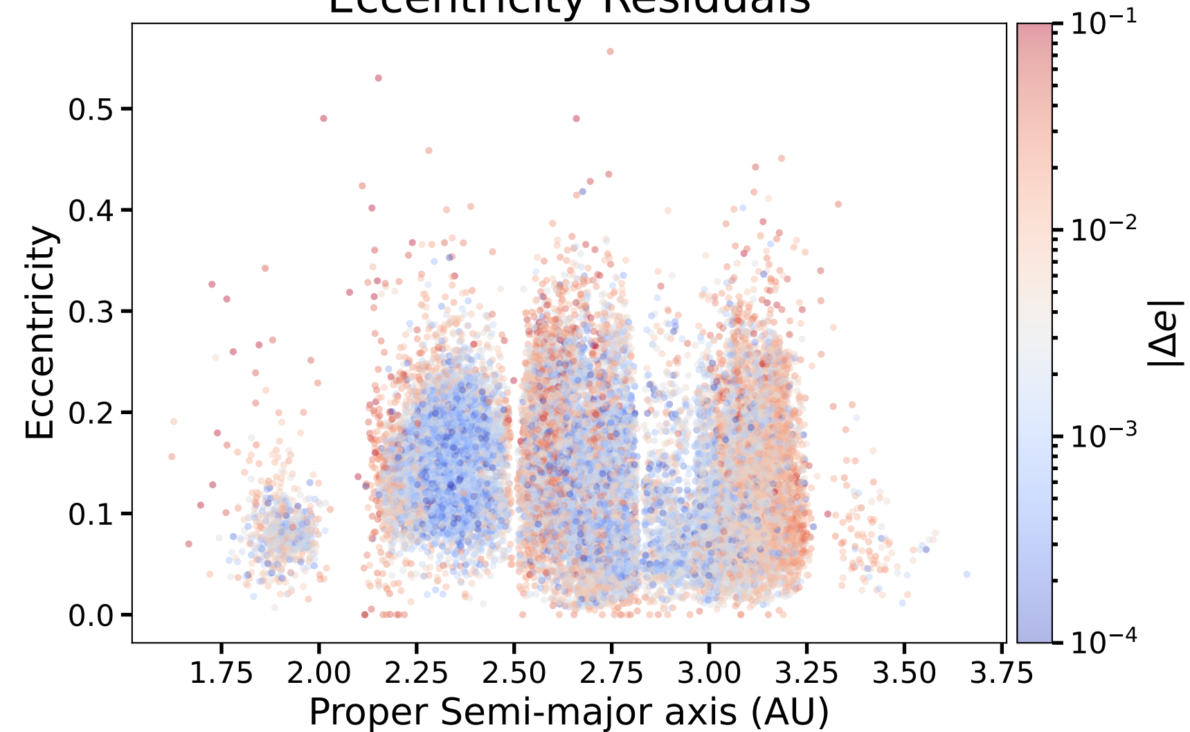
Eccentricity Residuals
