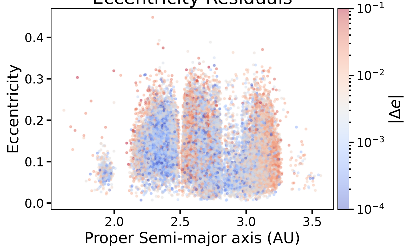
Eccentricity Residuals
