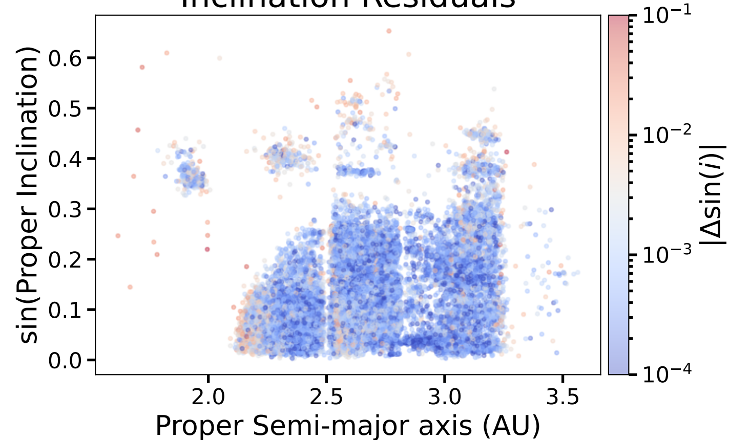
Inclination Residuals
