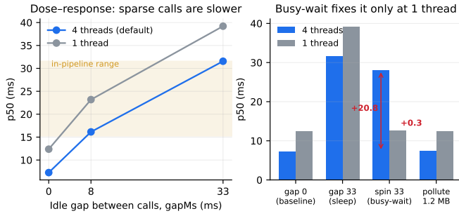
Fig. 6. Why an isolated benchmark is not the product-path cost. Left: raising the idle gap between calls from 0 to 33 ms raises the median from 7.26 ms to 31.56 ms, and the upper end of that range coincides with the in-pipeline measurements. Right: a busy-wait of the same duration does not recover the loss at four threads (+20.8 ms) but almost fully recovers it at one (+0.29 ms), separating frequency scaling from thread-pool wake-up.
