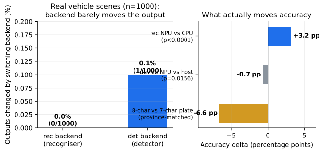
Fig. 3. Left: over 1,000 real vehicle scenes, switching a role’s backend almost never changes the output. Right: the quantities that do move accuracy, including one that moves it in the opposite direction.
