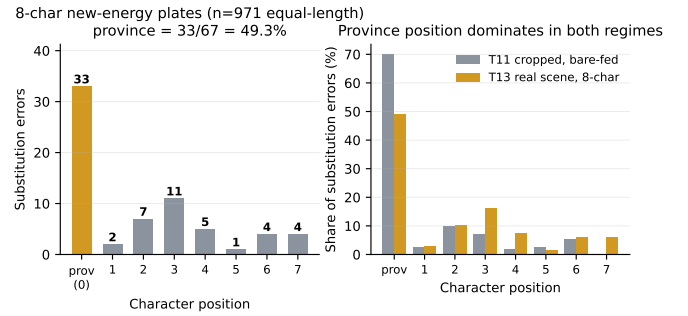
Fig. 4. Substitution errors by character position. The province position dominates across regimes, plate lengths and backends.
