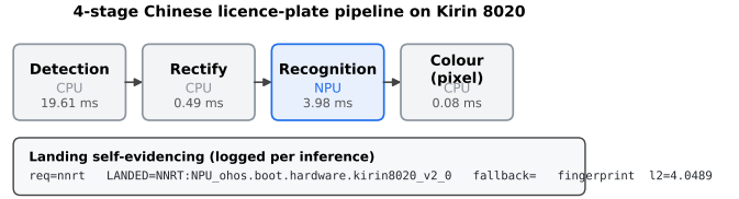
Fig. 2. The four-stage pipeline and the per-inference landing record. Stage timings are from the production configuration on a detected frame (median).
