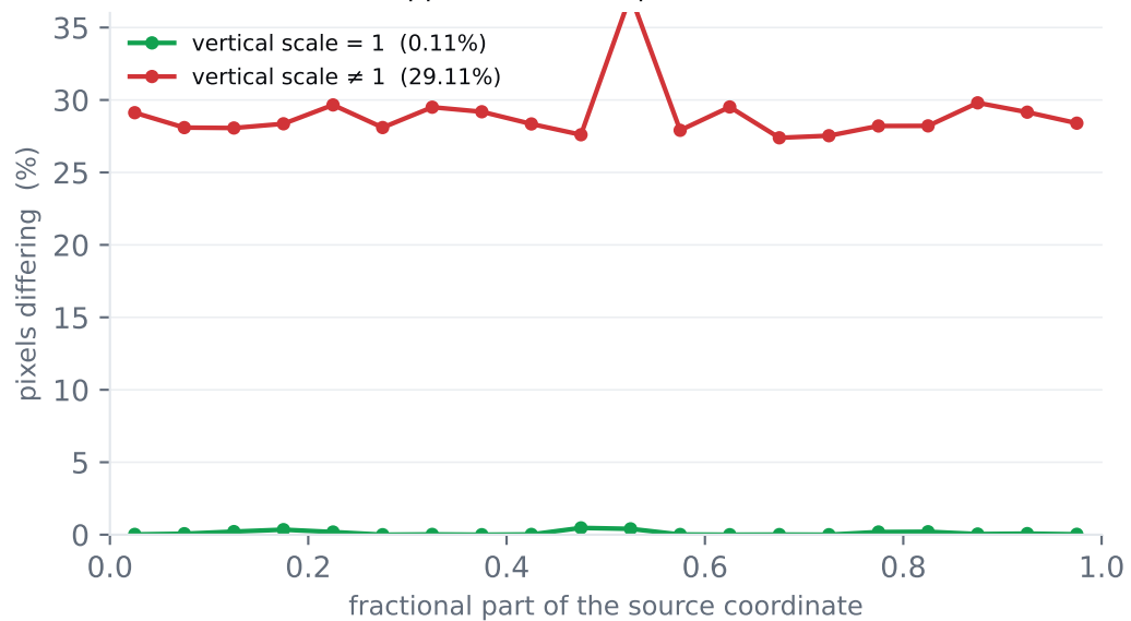
(b) shipped resize vs OpenCV, 135 scales
