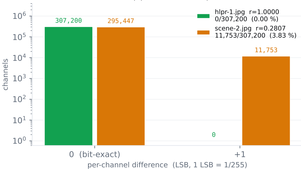
(a) real pipeline cases vs OpenCV
