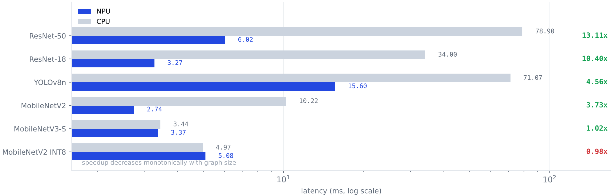
Kirin 8020: NPU vs CPU latency (P50, ms)
