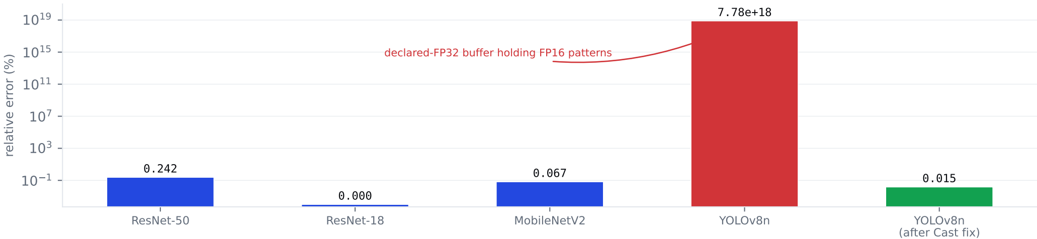
Output L2 relative error, NPU vs CPU
