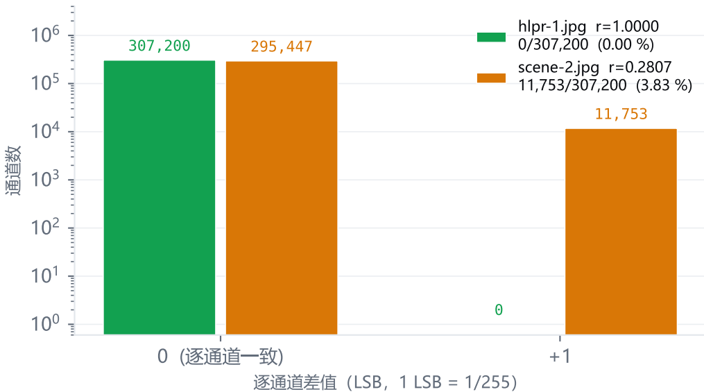
(a) 真实流水线样本 vs OpenCV
