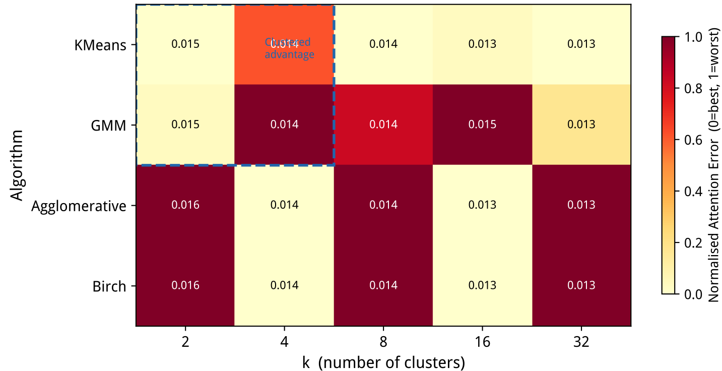
Method D: Attention Error by Algorithm & k (rank = 8)
