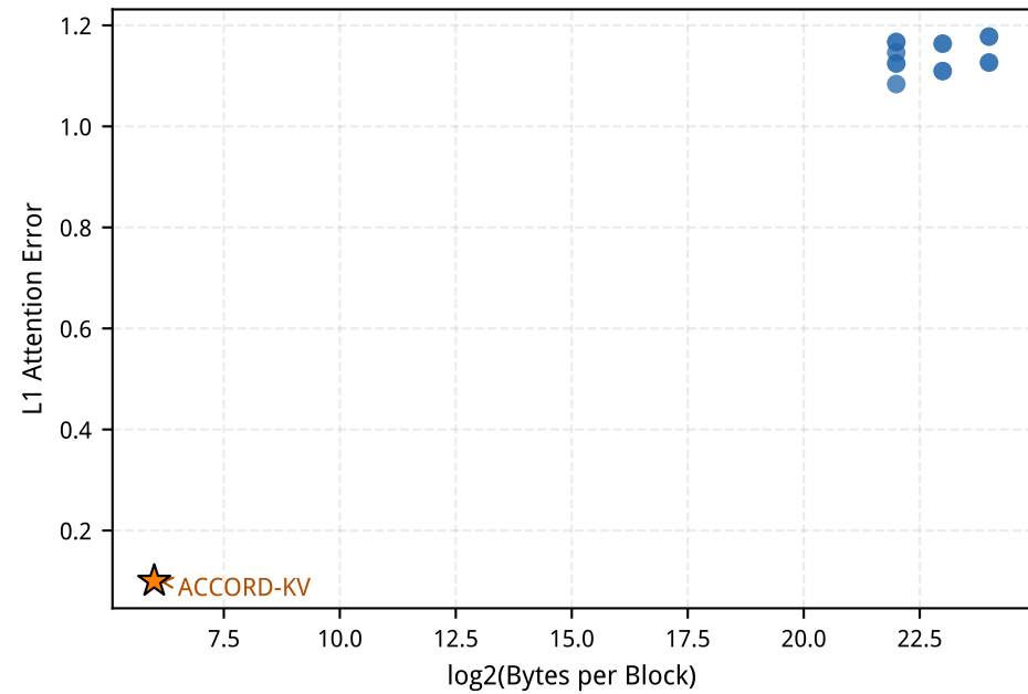
Skewed Distribution
