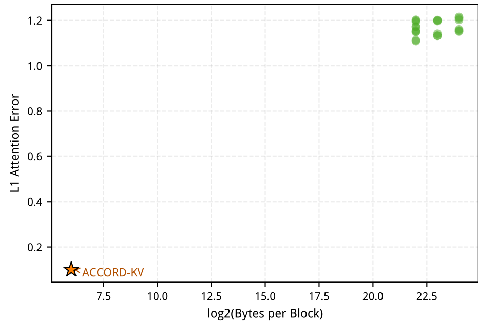
Uniform Distribution
