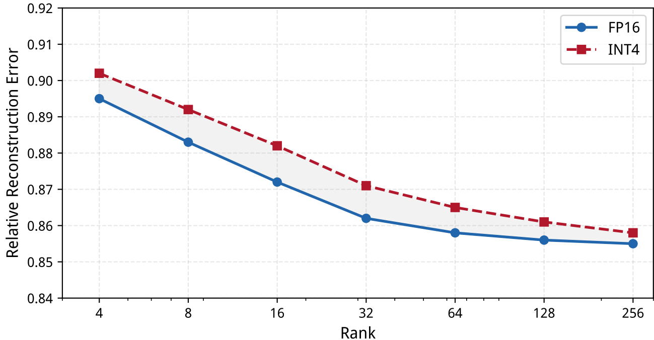
Relative Reconstruction Error vs. Rank (INT4)
