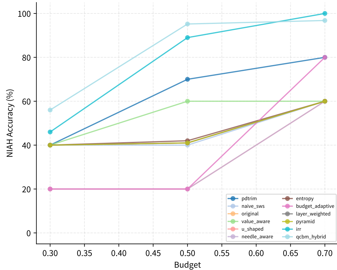
qwen-7b (seq=4096)
