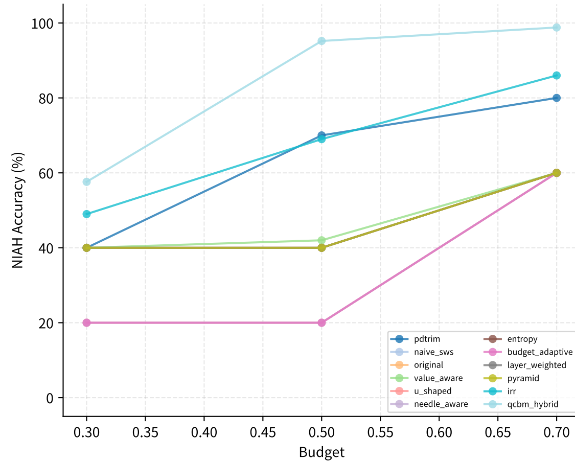
mistral-7b (seq=4096)
