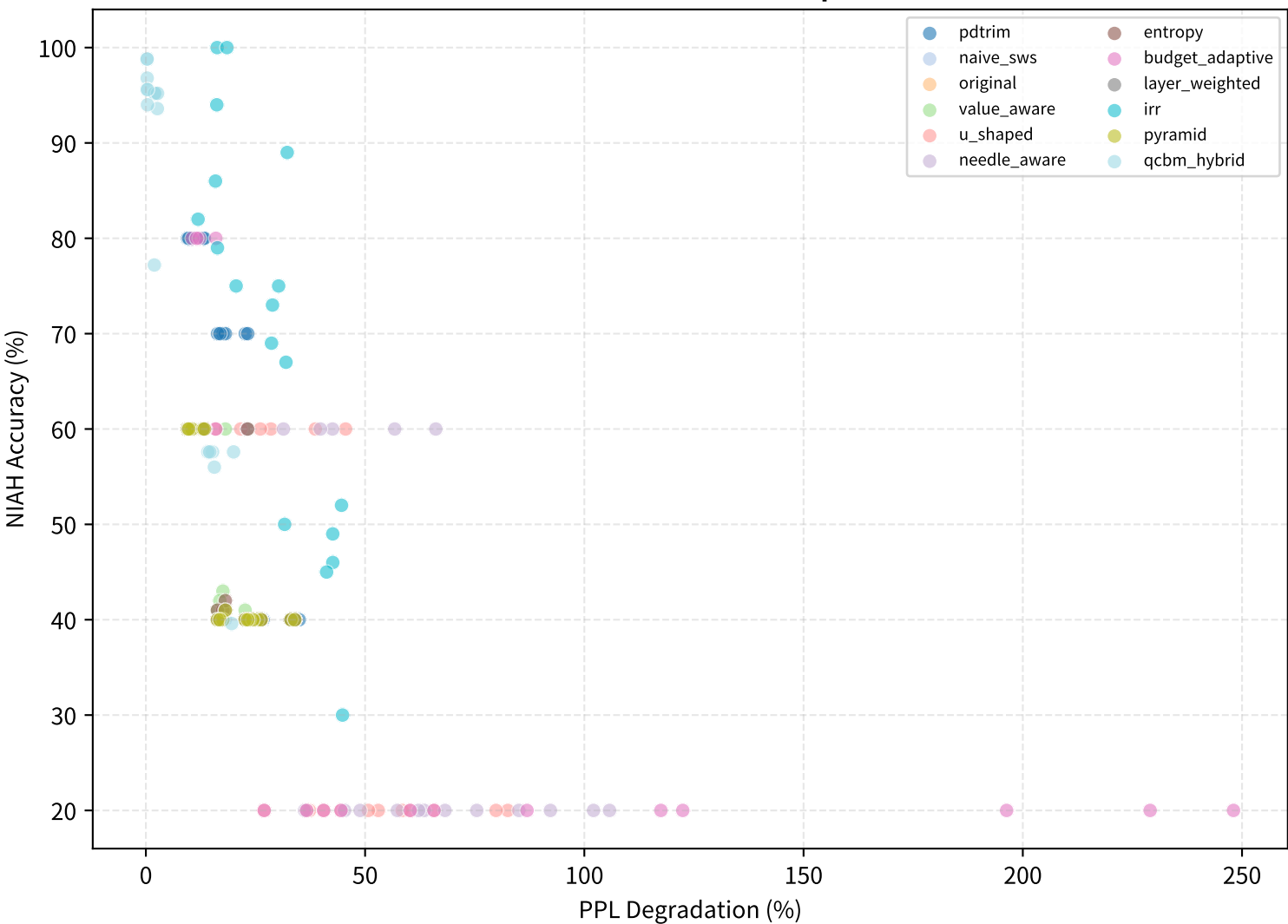
PPL vs NIAH: Formula Comparison
