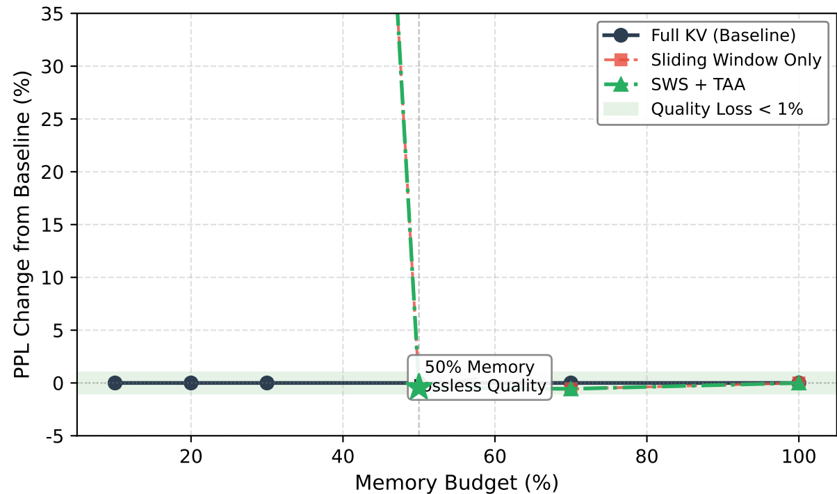
Figure 1: Memory-Quality Pareto Frontier
