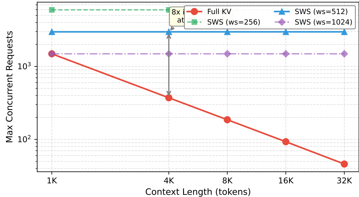
Figure 5: Concurrent Request Capacity
