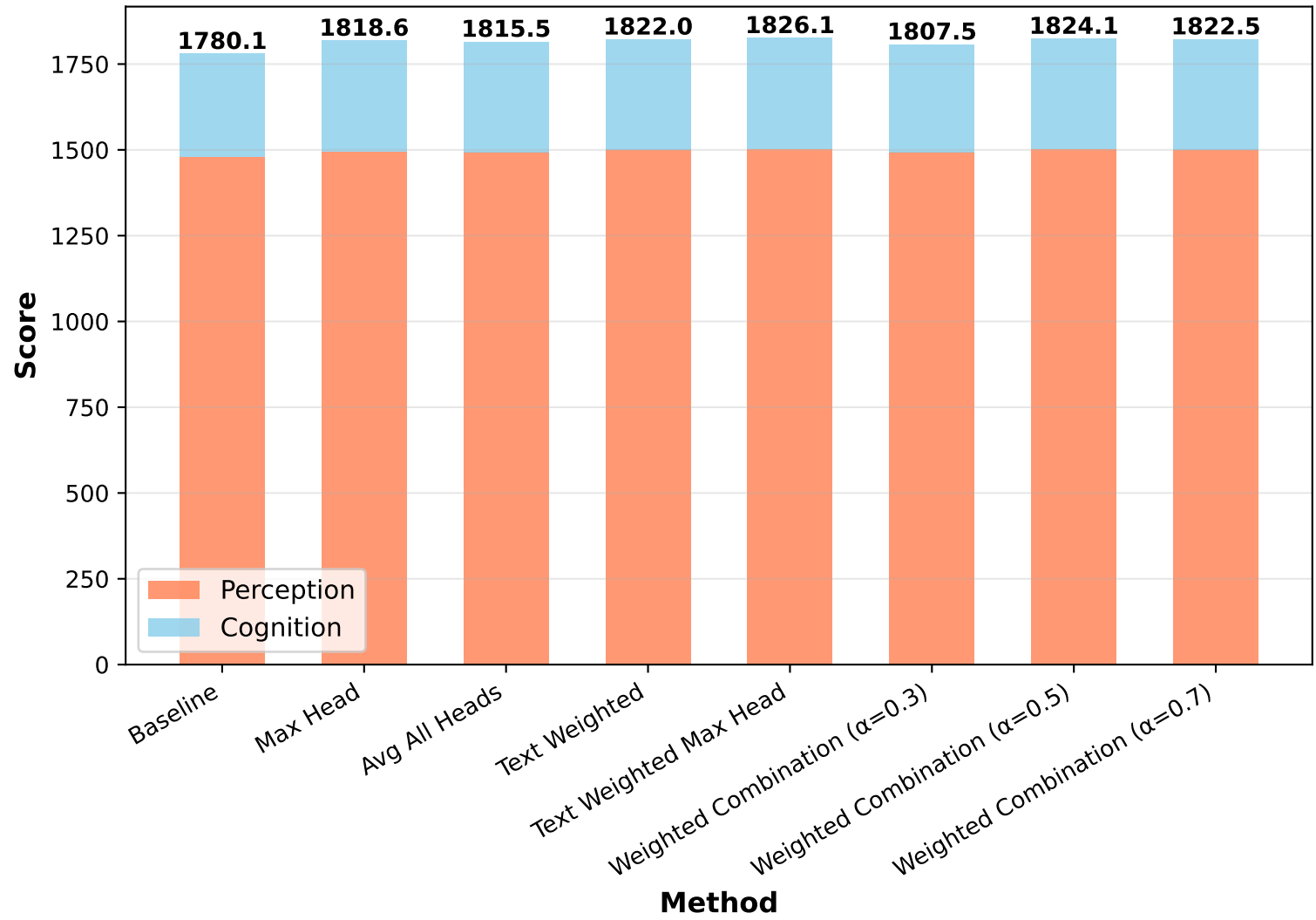
Perception vs Cognition Score Breakdown
