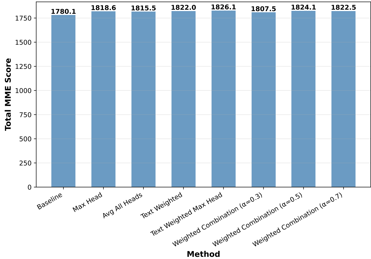
MME Total Score Comparison
