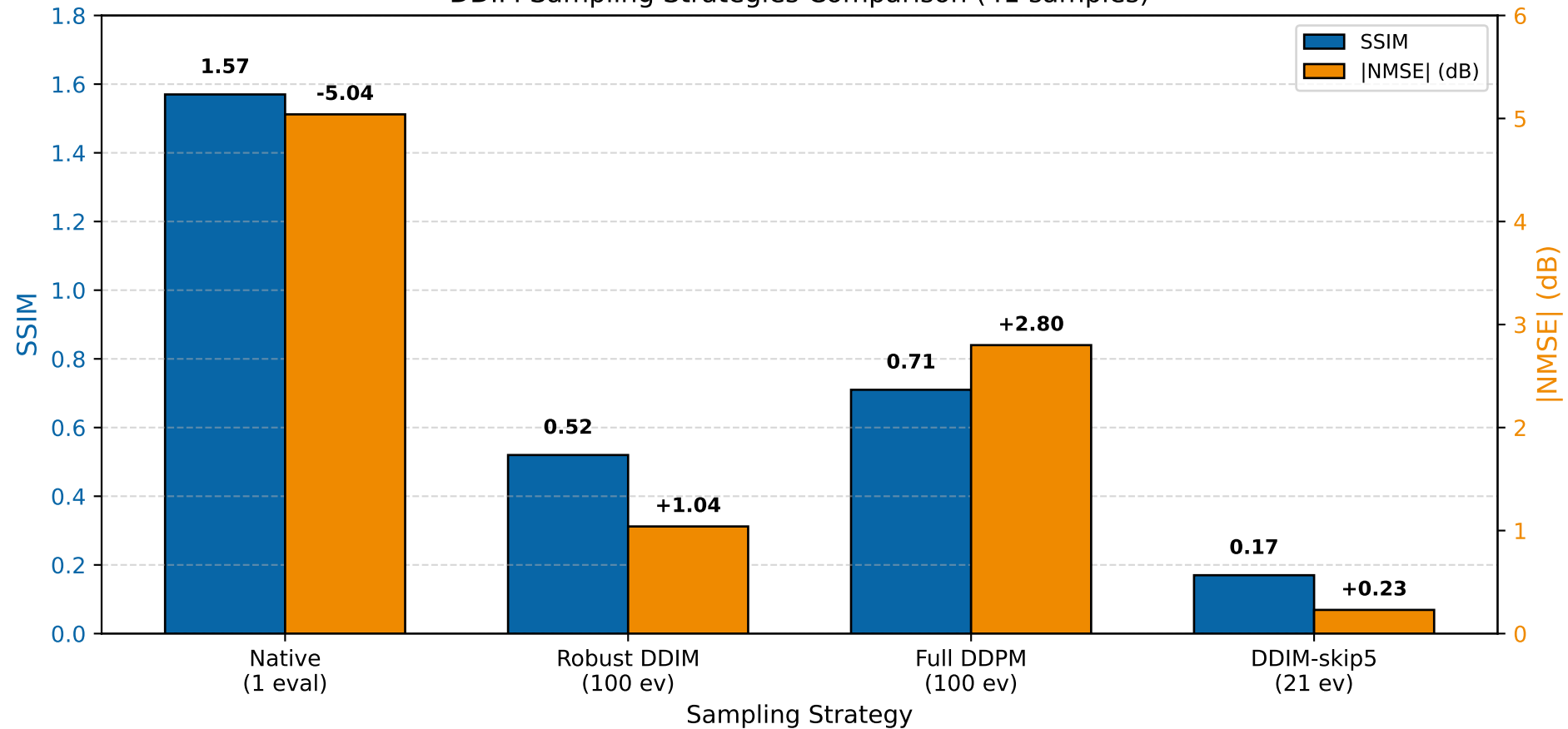
DDIM Sampling Strategies Comparison (41 samples)
