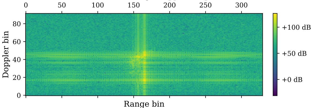
Real FMCW Range-Doppler Map
