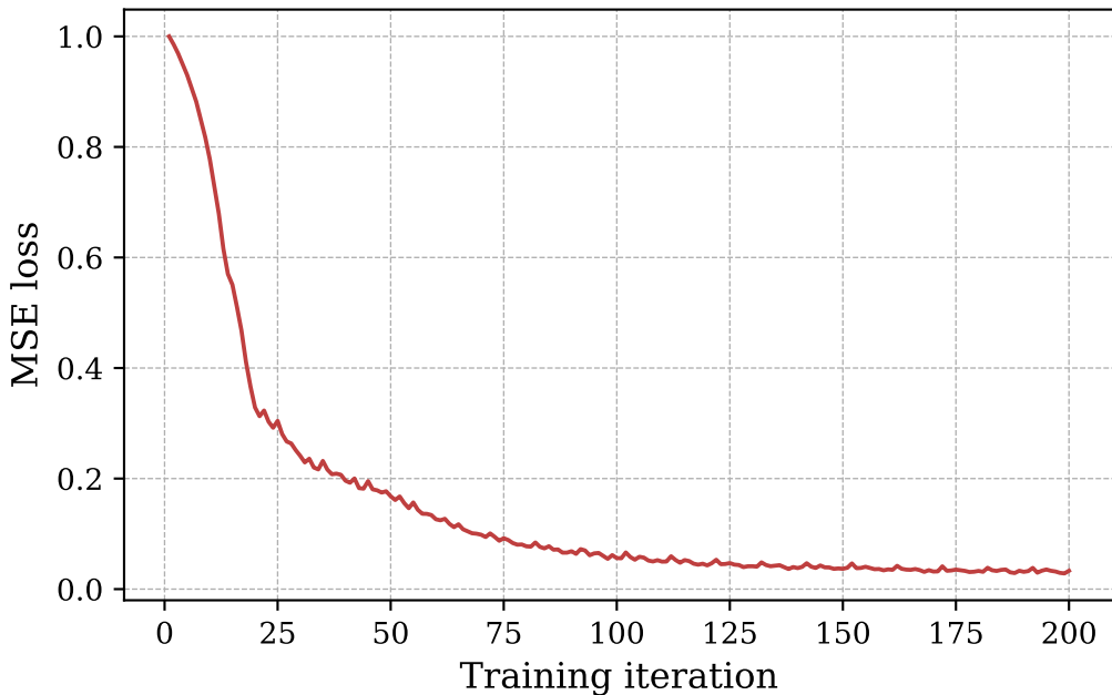
Small-scale training loss curve (b=4, hidden=64, iters=200)
