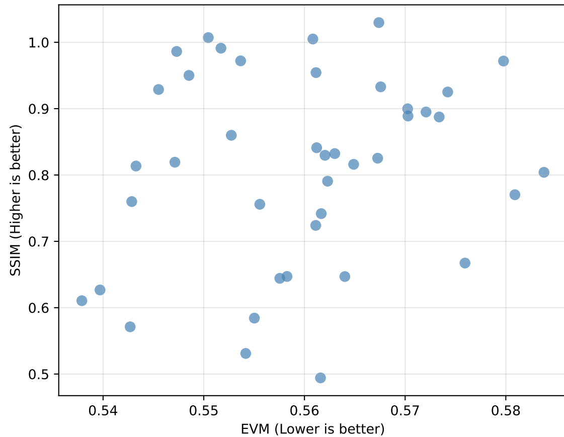
EVM vs SSIM Trade-off
