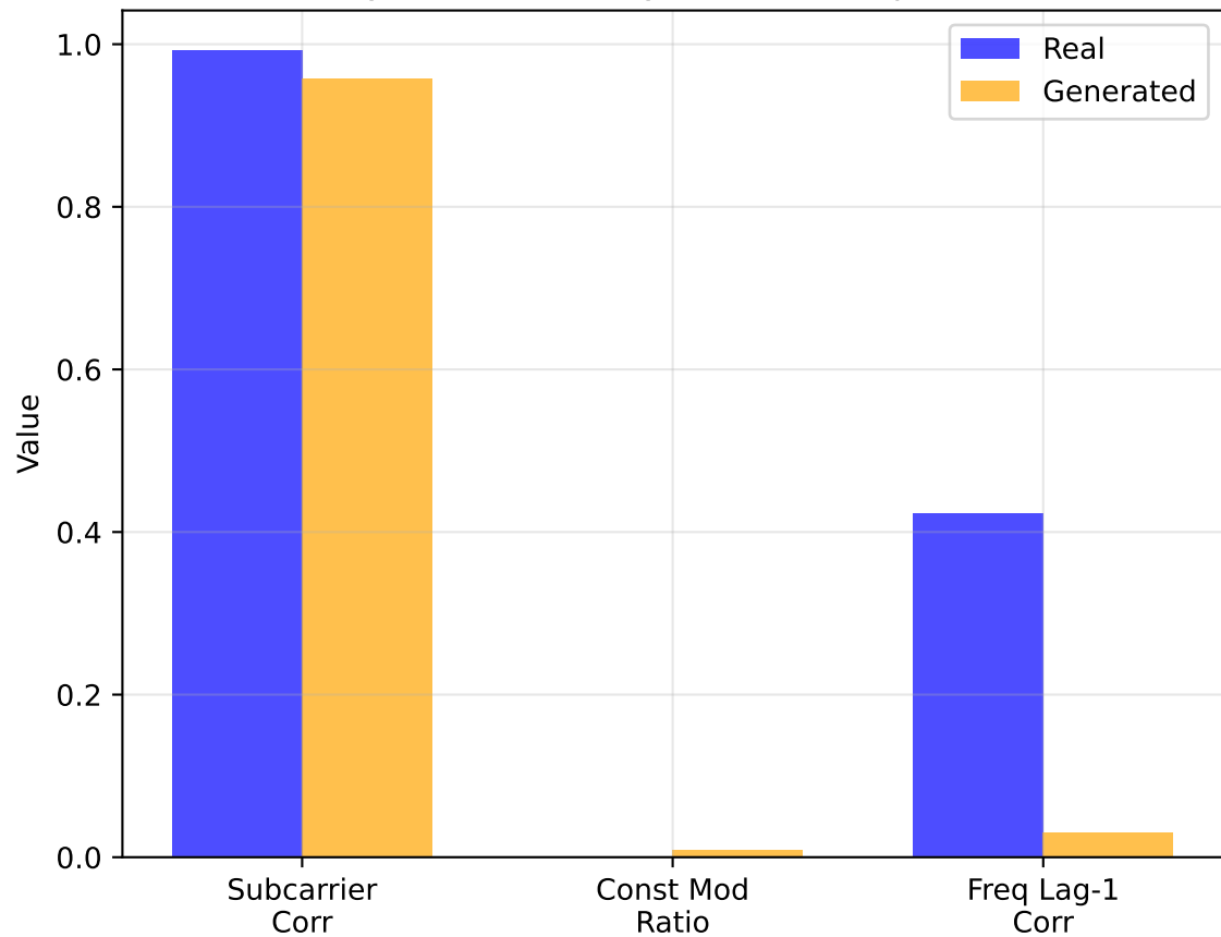
Physical Plausibility Metrics Comparison
