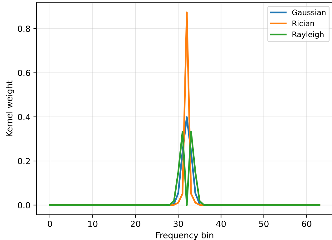
(a) Frequency-domain Blur Kernels Compared
