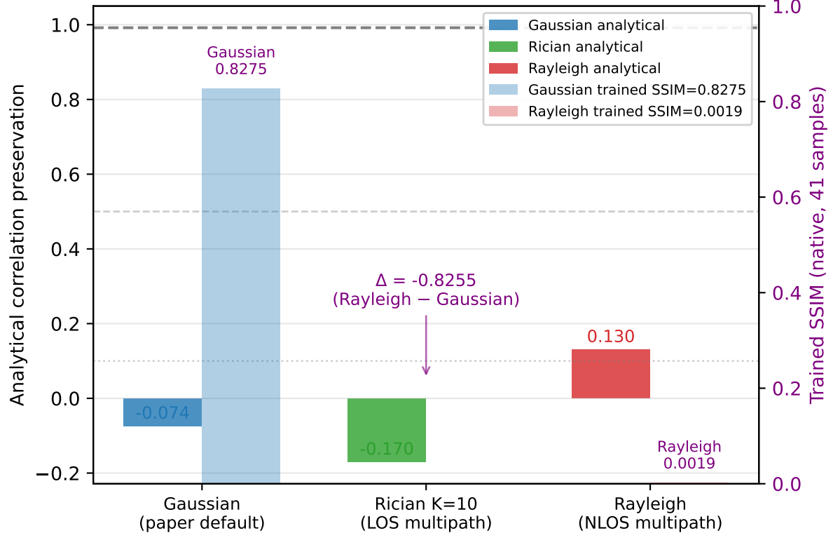
(b) Analytical vs. Trained SSIM (4 blocks / 64 / 100 iters)
