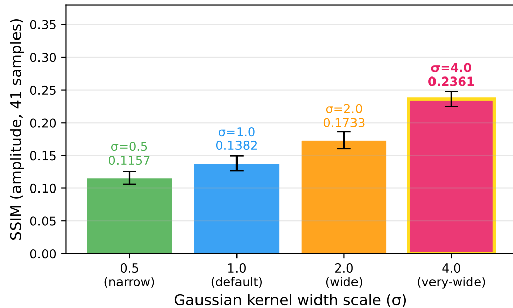
(a) SSIM vs Gaussian Kernel Width
