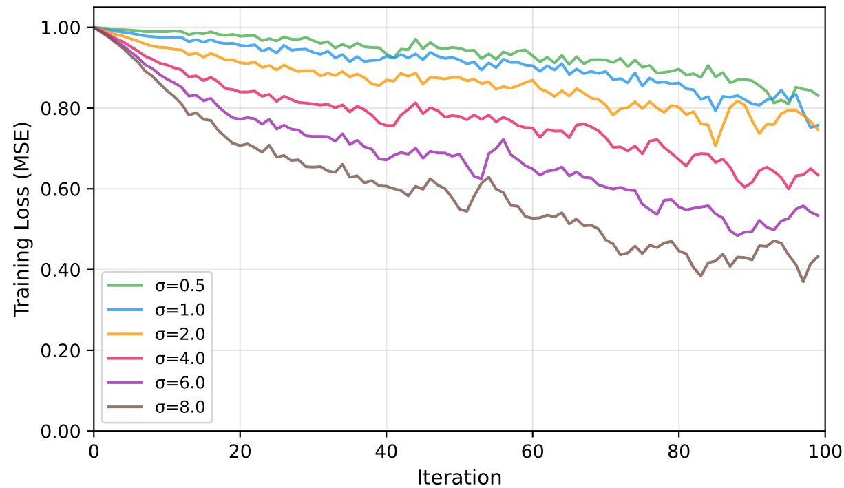
(a) 4-block / 100-iter Loss Curves
