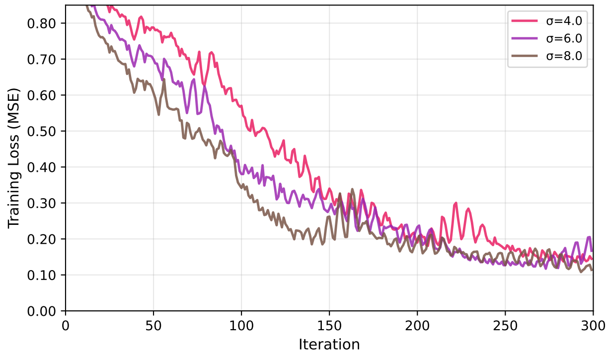
(b) 8-block / 300-iter Loss Curves
