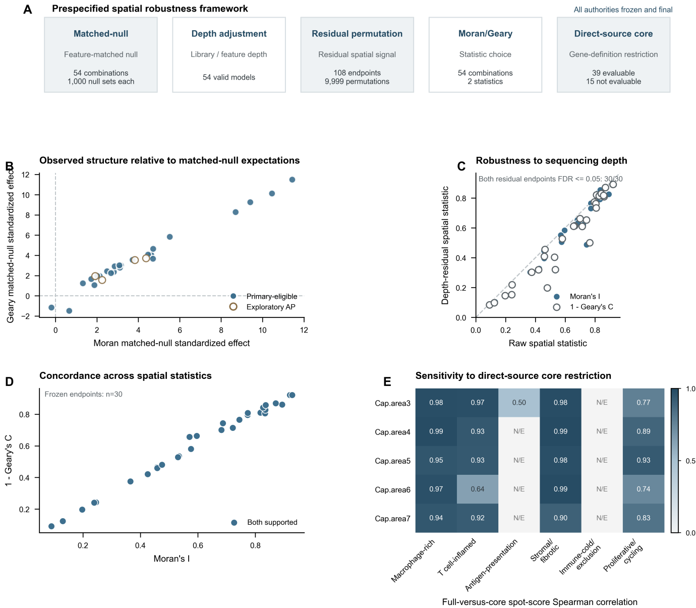
Supplementary Fig. S5 | Robustness and sensitivity analyses of spatial continuous-program structure
