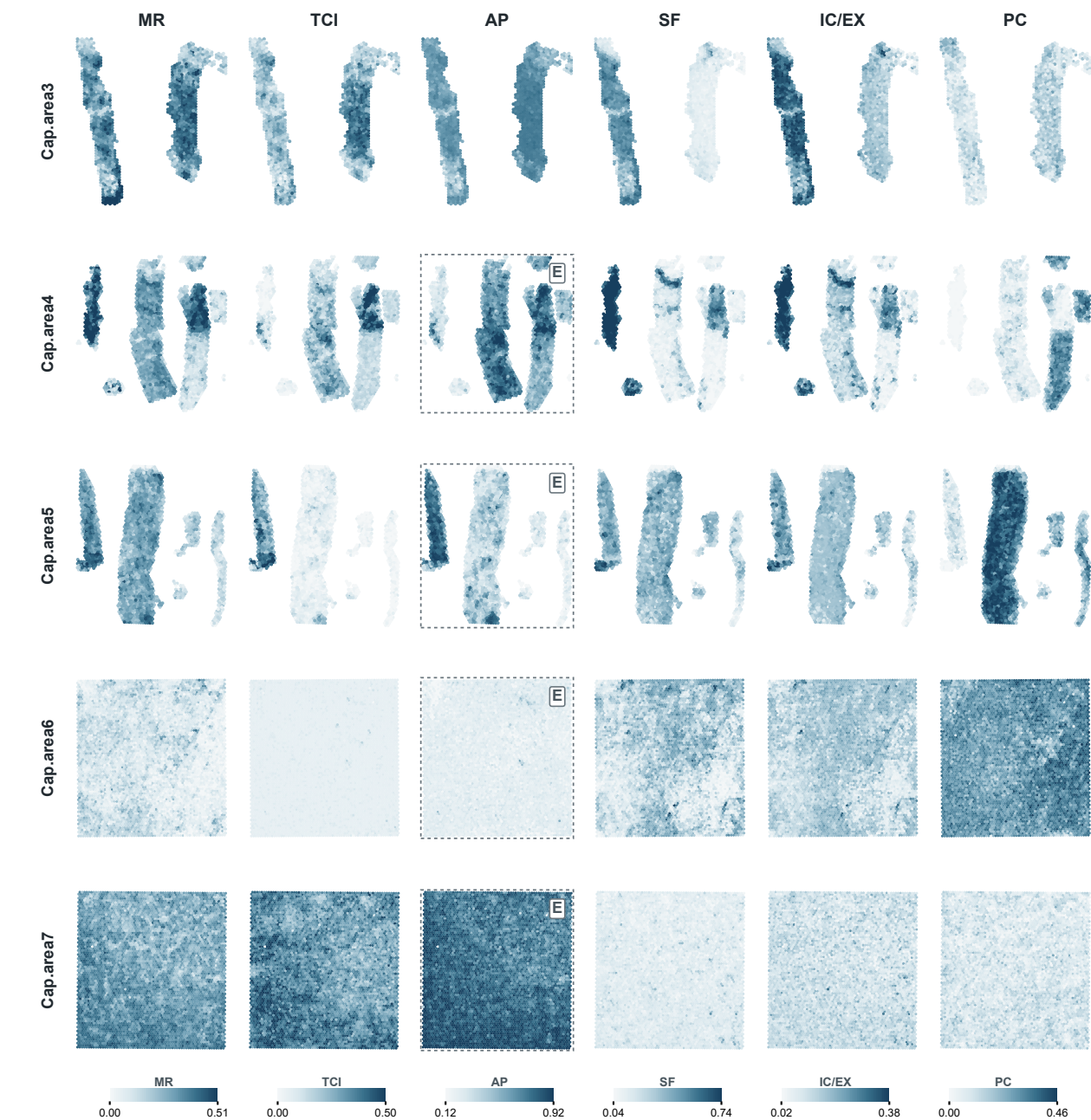
Supplementary Fig. S4 | Canonical UCell spatial distributions across five primary DLBCL capture areas
