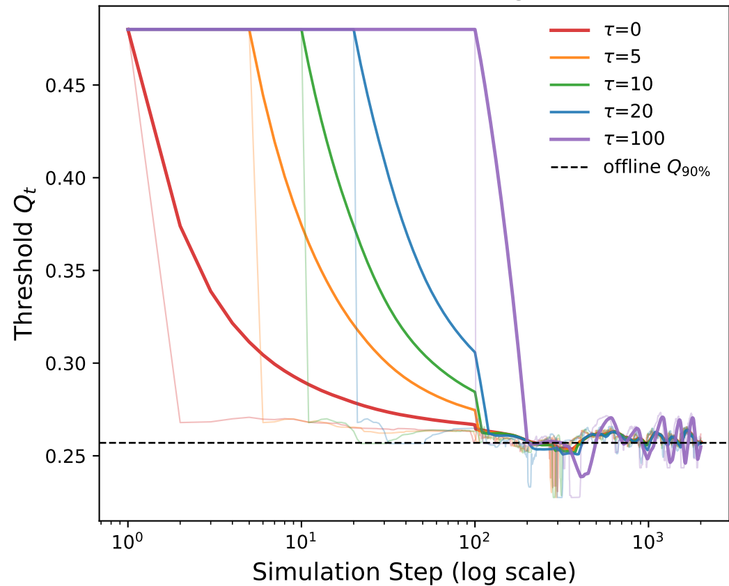
(a) Threshold Convergence
