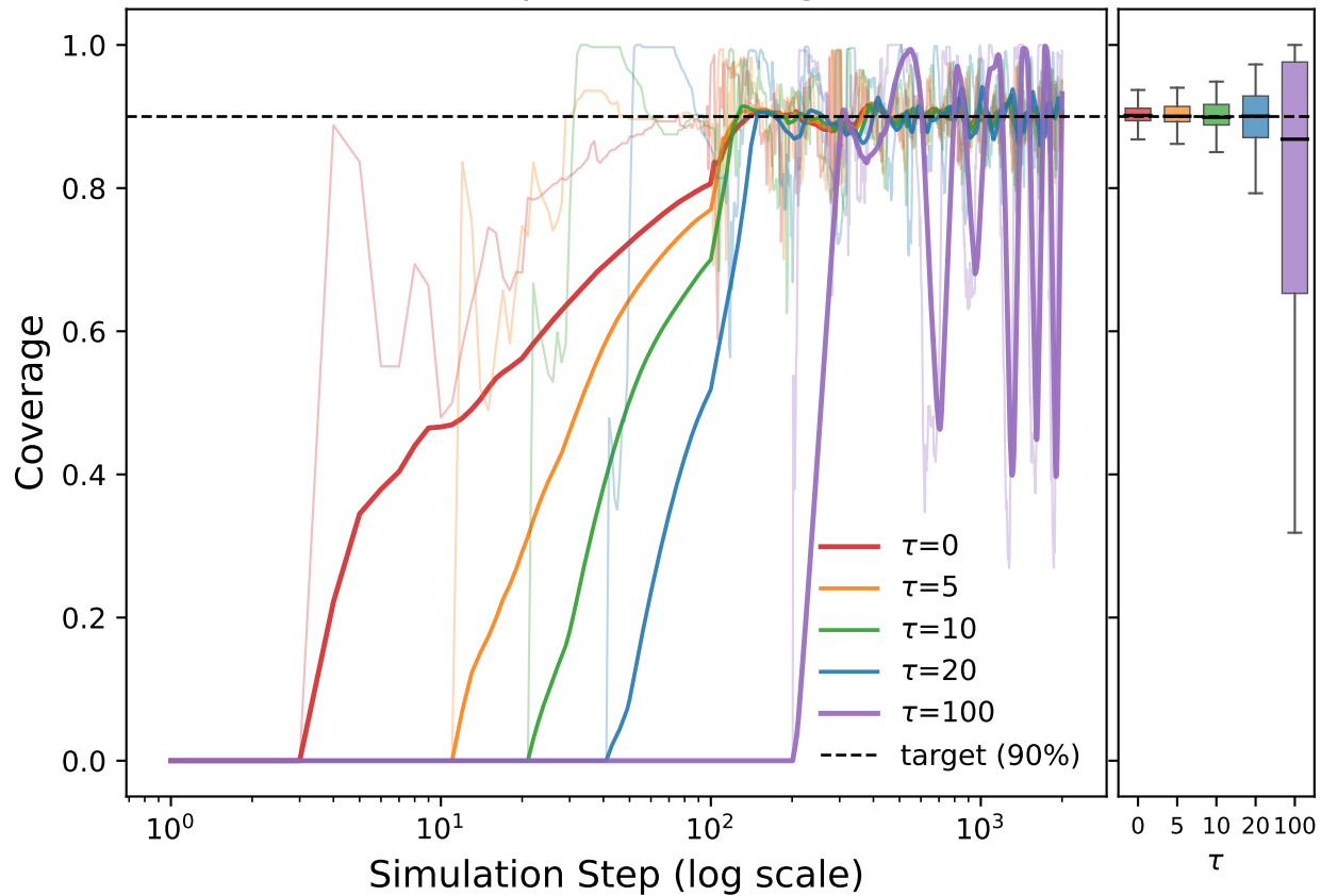
(b) Empirical Coverage
