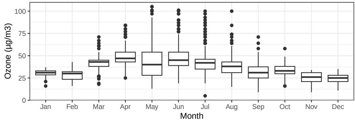
Figure 1: Monthly Ozone (2018).
