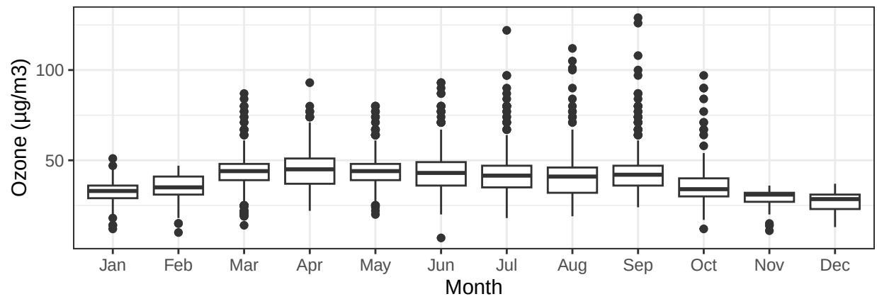
Figure 2: Monthly Ozone (2019).
