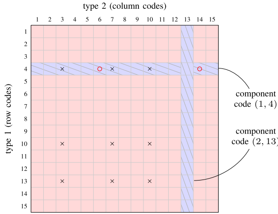
Fig. 1. PC array for a length-15 component code. Two particular component codewords are highlighted. The black crosses correspond to a minimal-size stopping set when t = 2 . Red circles indicate a miscorrection, see Example 3.
