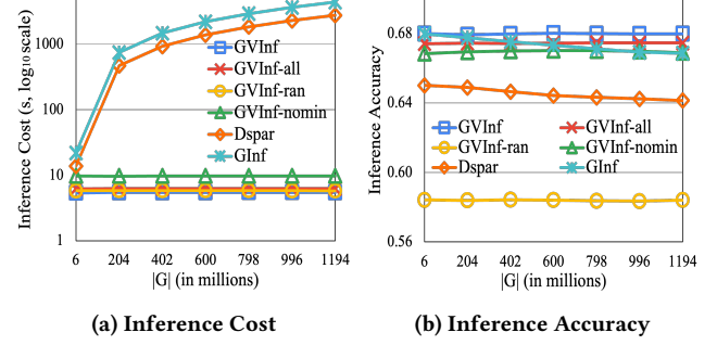
Figure 12: The Impact of |G| on View based graph inference.
