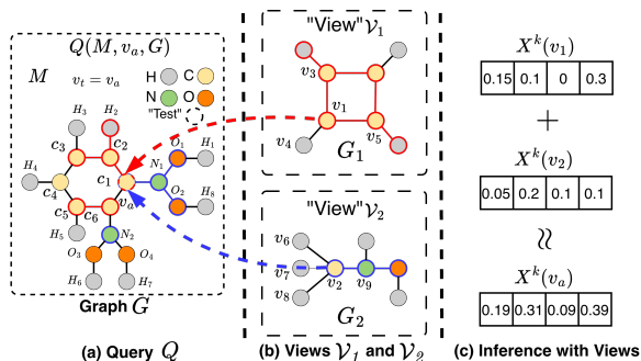
Figure 1: Approximate Evaluation of an Inference Query Q over Target Molecular Graph G Using “Views” V_1 and V_2 .
