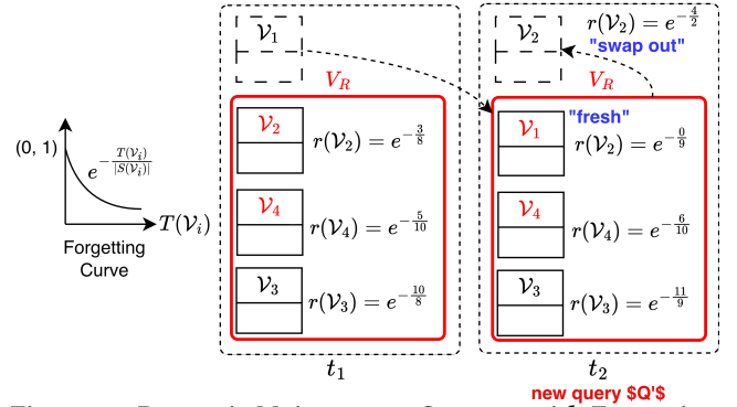
Figure 12: Dynamic Maintenance Strategy with Forgetting Mechanism. Discarding stale views in \mathcal{V} and serves only the current “fresh” subset \mathcal{V}_R .
