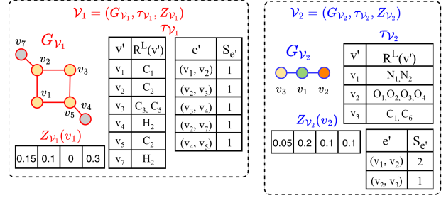
Figure 4: Extended GMVs \mathcal{V}_1 and \mathcal{V}_2 .
