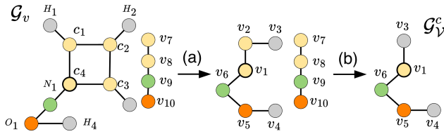
Figure 7: Algorithm GVMin.
