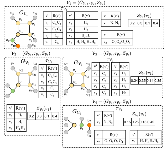
Figure 6: View Selection for Graph Inference. Of the four GMVs \mathcal{V}_1, \mathcal{V}_2, \mathcal{V}_3 , and \mathcal{V}_4 , \mathcal{V}_1 completely covers Q while \mathcal{V}_2, \mathcal{V}_3 , and \mathcal{V}_4 covers Q partially.
