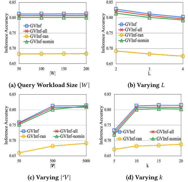
Figure 11: Inference Accuracy of View-based Inference.
