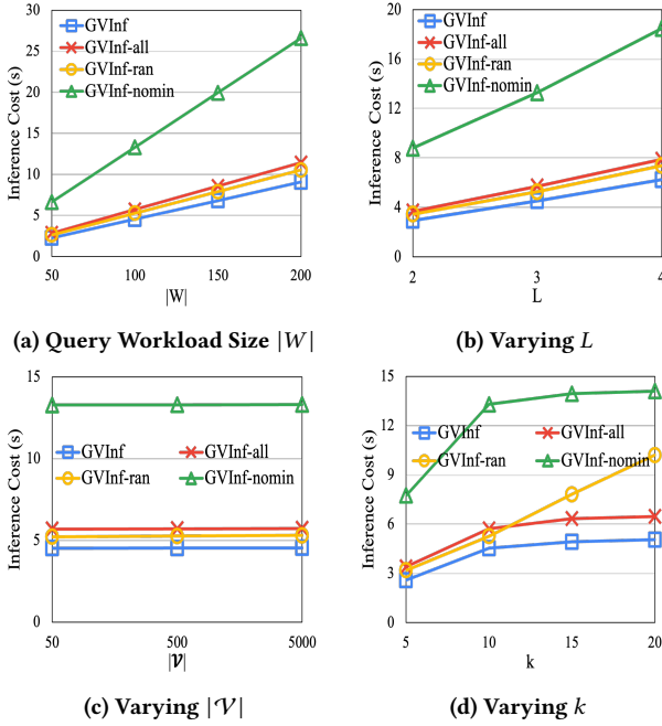
Figure 10: Inference Costs of View-based Inference.
