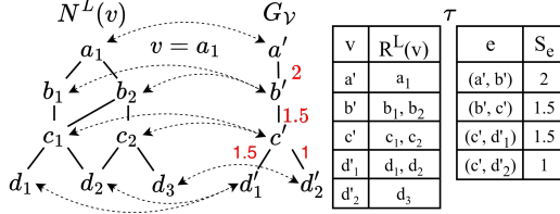
Figure 4: A illustration of View-based Inference (memory graph G_V simulates N^L(v) with L = 3 where view \mathcal{V}(G_V) covers global query Q = (M^L, G, v) ).
