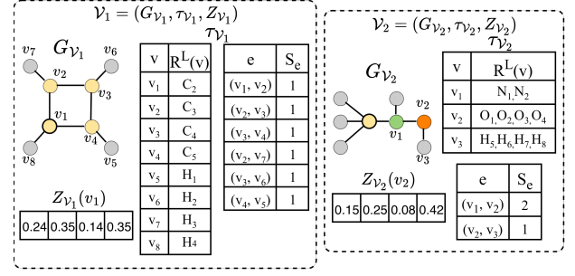
Figure 3: Extended GMVs \mathcal{V}_1 and \mathcal{V}_2 .
