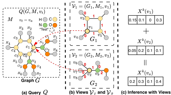
Figure 1: GNNs-based Molecular Property Prediction referring to “views” \mathcal{V}_1 and \mathcal{V}_2 only to answer inference query Q .
