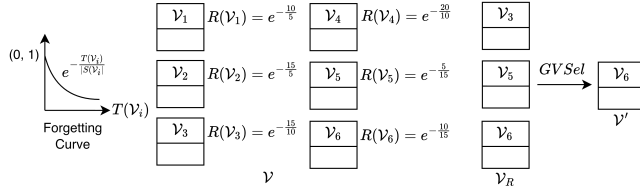
Figure 13: Dynamic Maintenance Strategy with Forgetting Mechanism. Discarding stale views in \mathcal{V} and serves only the current “fresh” subset \mathcal{V}_R .
