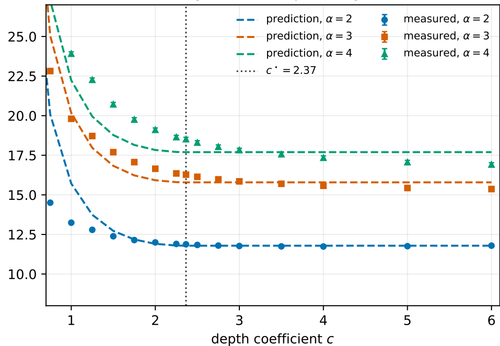
Logarithmic-depth range
