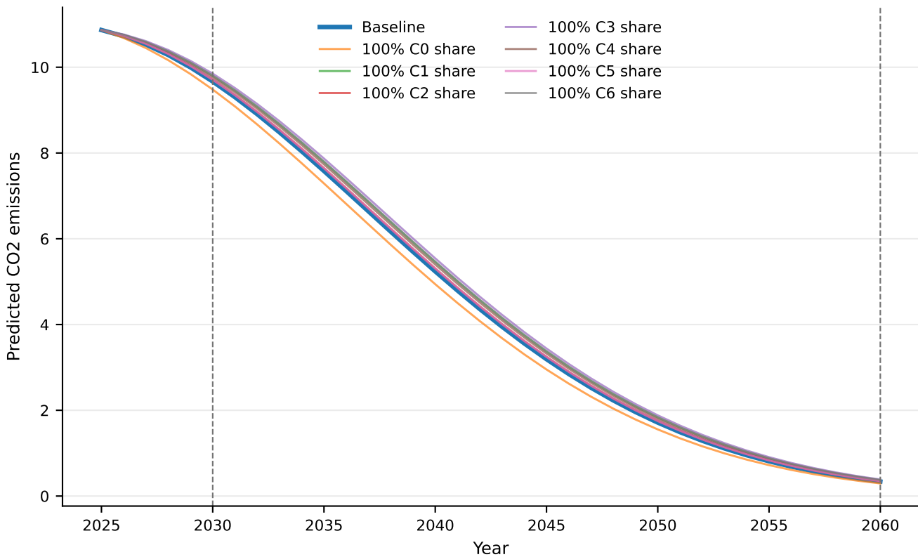
National CO2 forecasting scenarios
