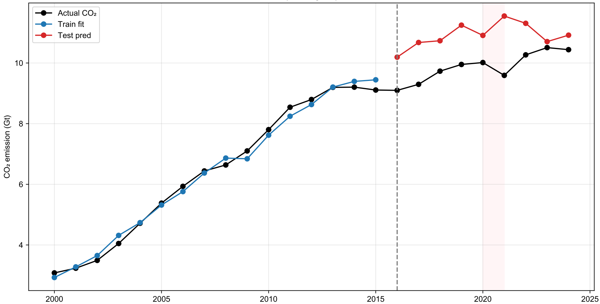
ElasticNet CO 2 Fit (No Regime) — Test R 2 = -5.07
