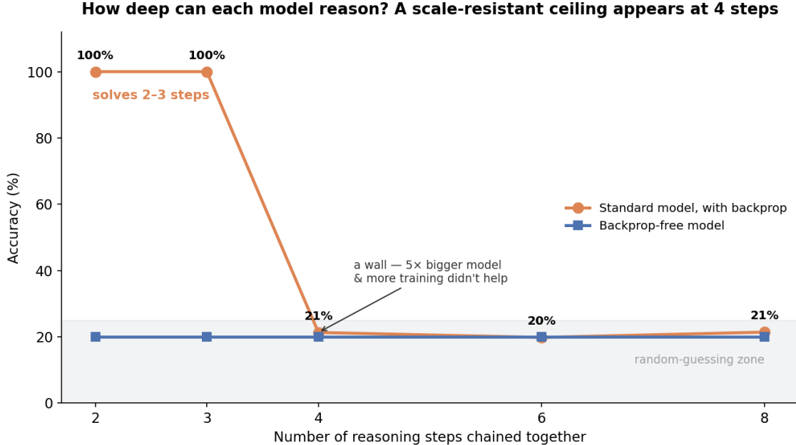
Figure 3: Reasoning-depth wall. The control solves 2–3 chained steps but stalls at k \geq 4 , unchanged by a 5\times larger model and longer training.
