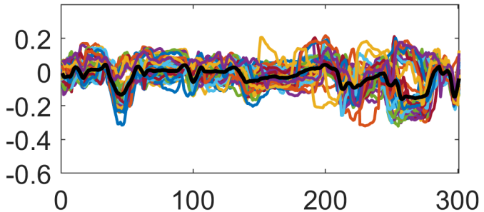
Reconstructed \tilde{\mathbf{W}}_{\alpha_m}
