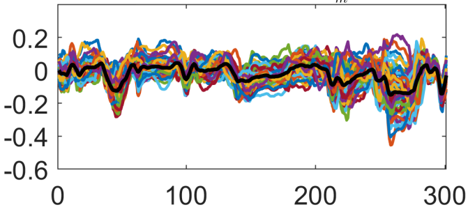
Simulated \mathbf{W}_{\alpha_m}^*
