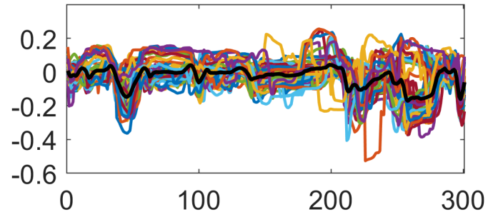
Original \mathbf{W}_{\alpha_m}
