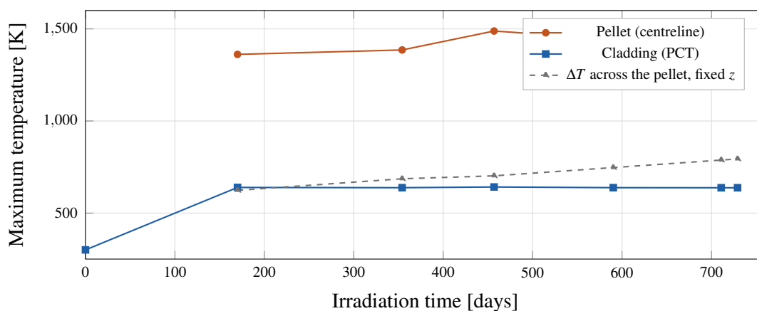
Figure 4.1: Evolution of the temperatures over the cycle. The two upper curves are maxima taken over the whole rod; the dashed curve is the centre-to-edge drop across the pellet at a fixed axial position, 0.45 m, where the local power stays constant to within 0.5 %.
