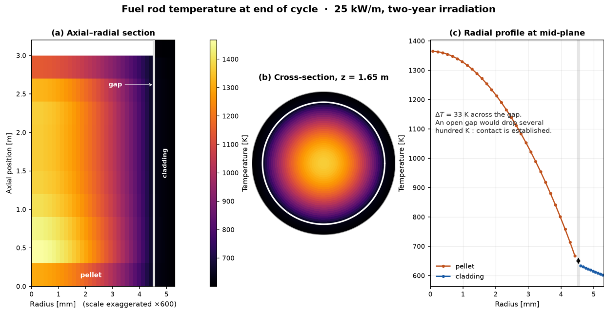
Figure 4.3: Temperature of the rod at end of cycle. (a) axial–radial section, radial scale exaggerated \times 600 ; the axial maximum sits near 0.5 m, following the cosine power profile. (b) cross-section at mid-plane. (c) radial profile at mid-plane, drawn separately because the cladding spans only 35 K against 870 K for the whole rod and is therefore flattened on a shared colour scale.
